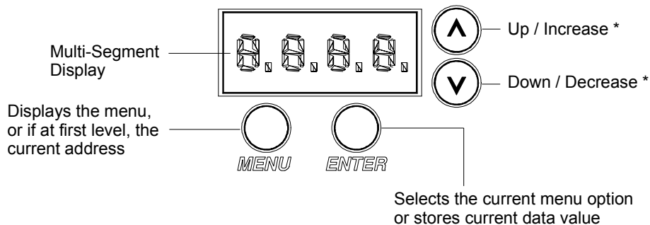
Figure 4-2: Controls Operation
