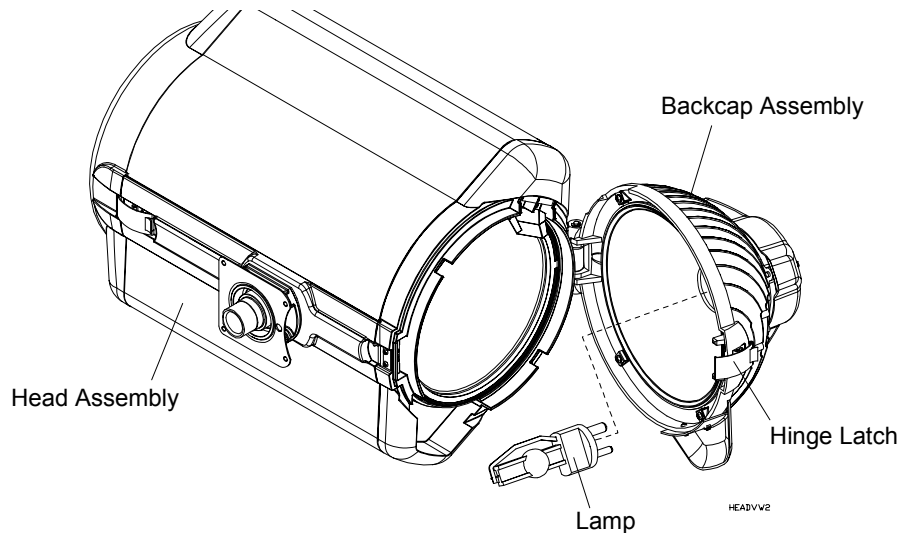
Figure 2-1: Installing/Replacing Lamp
