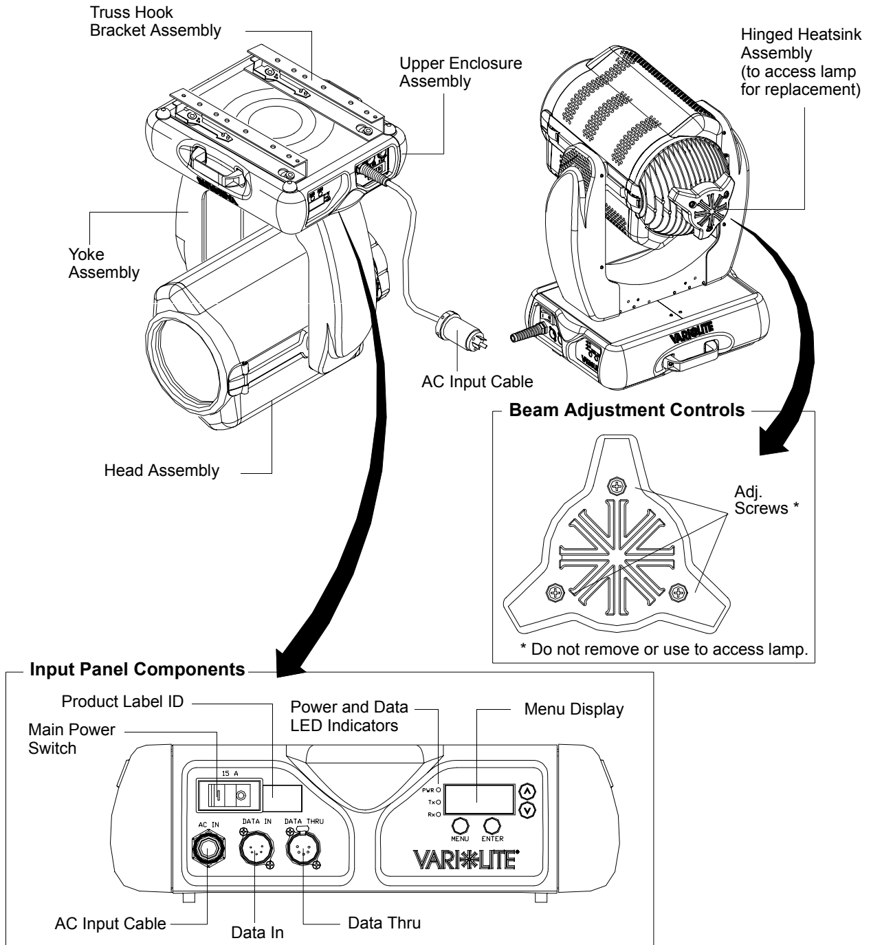
Figure 1-2: Luminaire Overview
