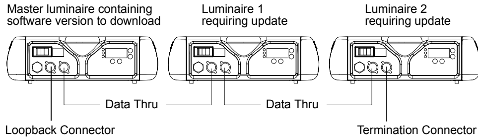
Figure 4-6: Test Setup
