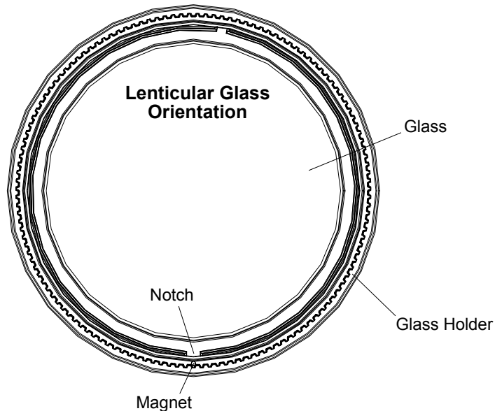
Figure A-3: Glass Alignment
