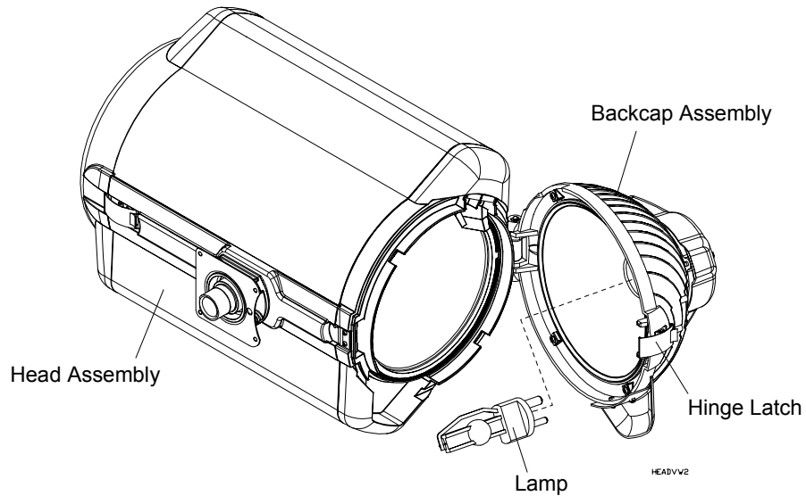
Figure A-1: Replacing Lamp
