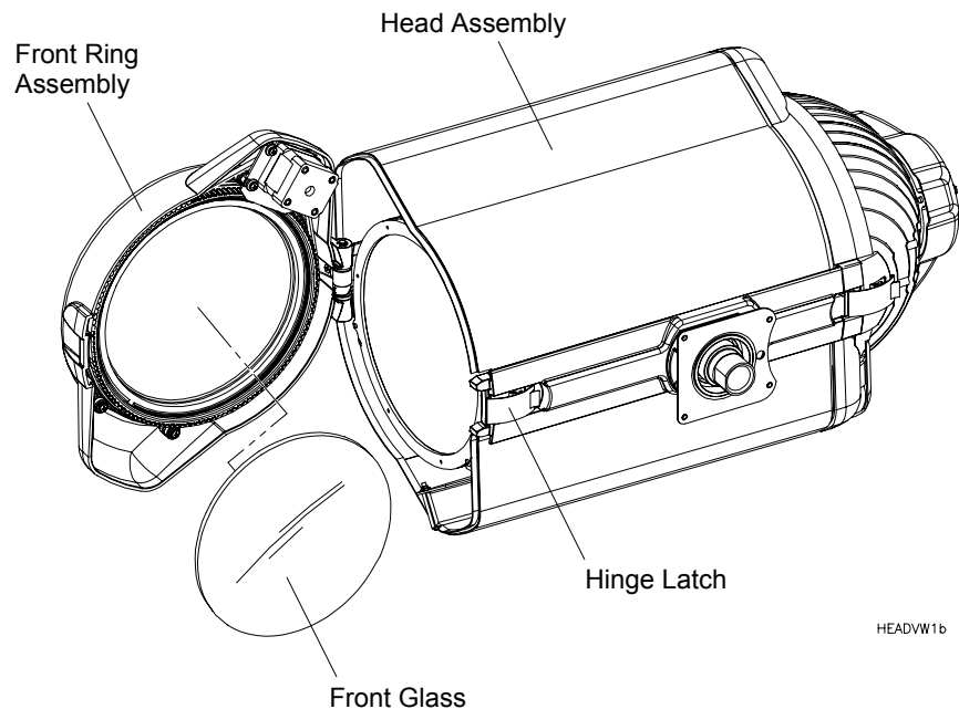
Figure A-2: Replacing Front Glass
